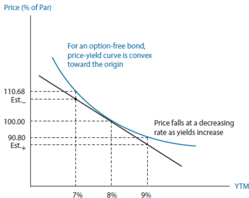
Figure 58.1: Price-Yield Curve for an Option-Free, 8%, 20-Year Semiannual-Pay Bond
