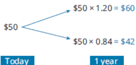
Figure 75.1: One-Period Binomial Tree
