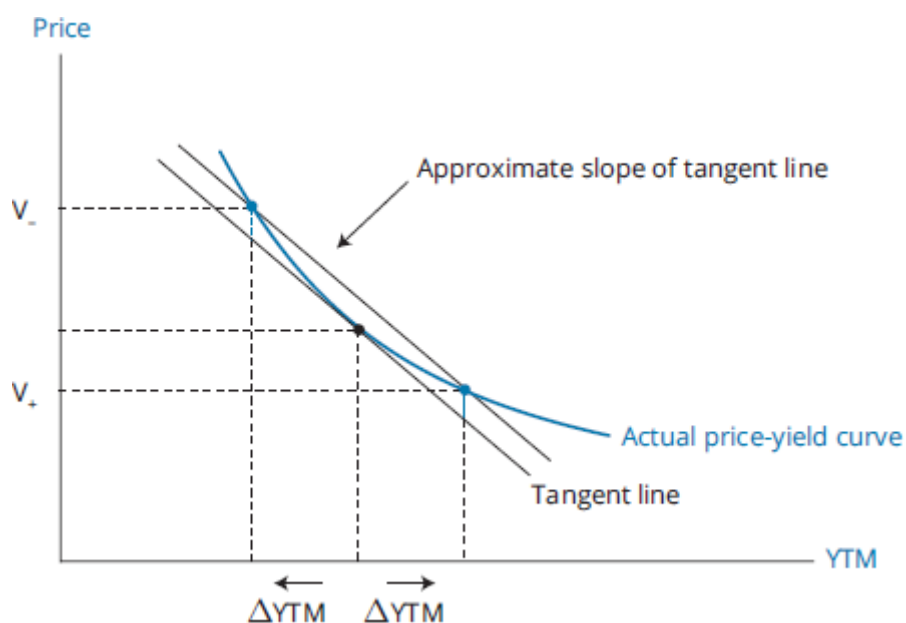
Figure 57.1: Approximate ModDur
