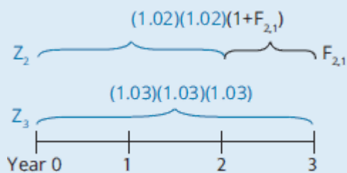
Figure 70.2: Implied Forward Rate
