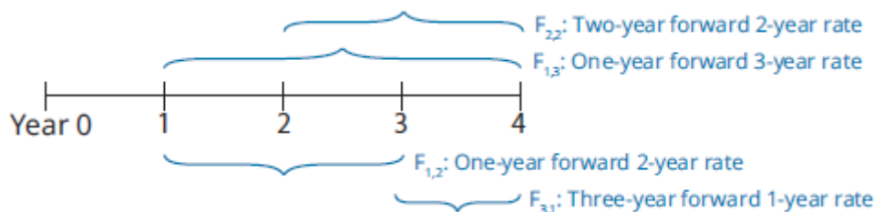
Figure 70.1: Forward Rates
